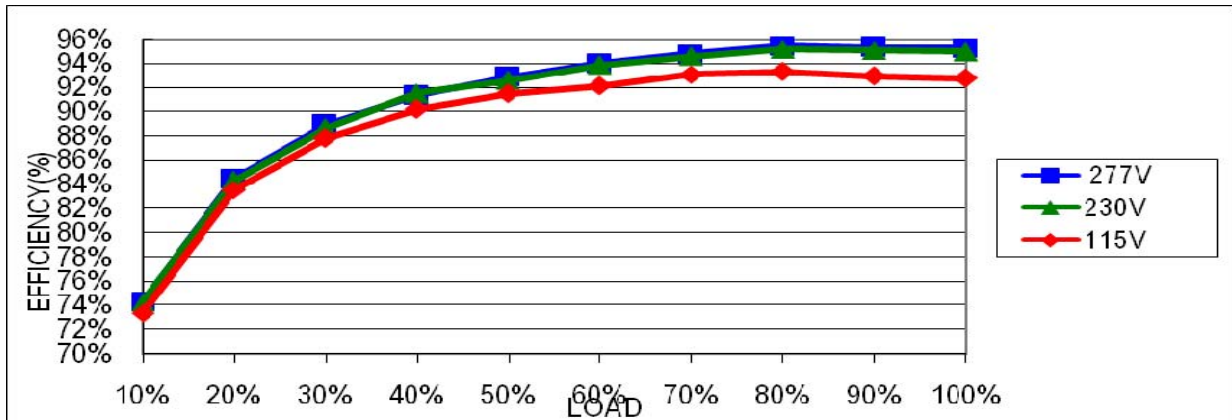
EFFICIENCY vs LOAD
