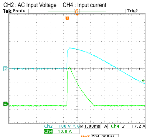
INPUT=115VAC/50HZ @ FULL LOAD
