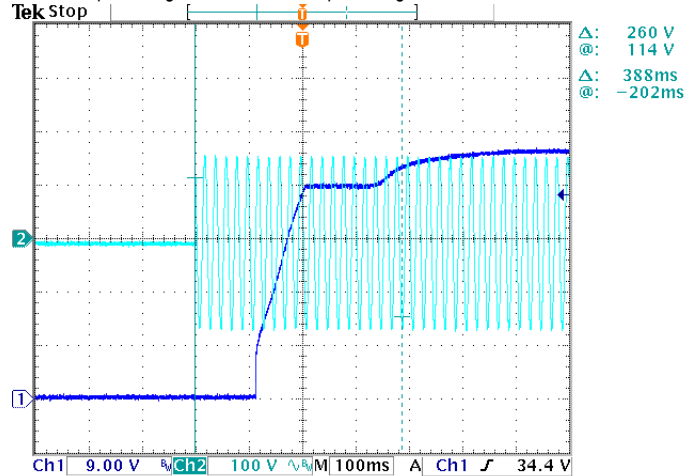
CH1: Output Voltage CH2: AC Input Voltage
