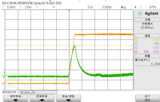
INPUT=24VDC @ FULL LOAD
