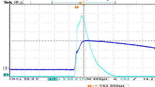
INPUT=115VAC/60HZ @ FULL LOAD
